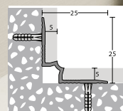
Terminal Degrau Stair nosing inner angle Perfilé nez-de-marche
